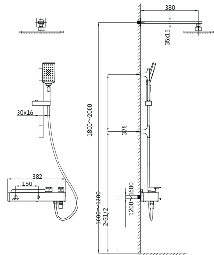
MARCO - 2 3 Function Rain Shower Chrome-White
